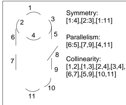
Figure 19: Sparse representation of a can with local curved lines corresponding to banana wavelets and lists of second order Gestalt relations between the local line segments (schematic).
