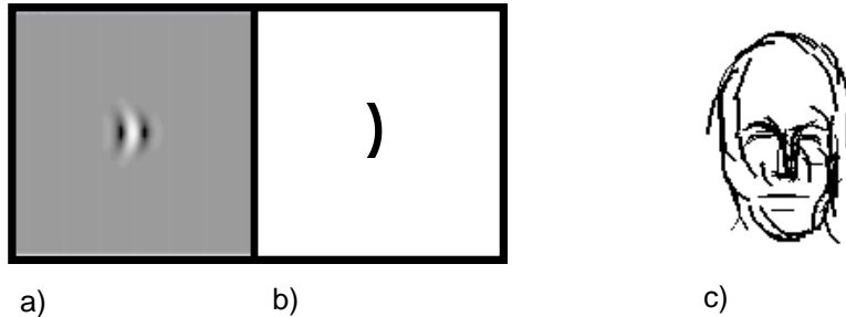
Figure 1: Path corresponding to a banana wavelet. a: Arbitrary wavelet. b: Corresponding path. c: Visualization of a representation of an object class. Gabor or Banana wavelets with lower frequencies are represented by line segments with larger width.
