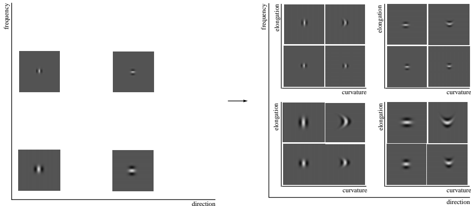
Figure 4: Relation between Gabor wavelets (left) and banana wavelets (right).
