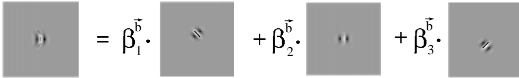
Figure 9: Approximation. The banana wavelet on the left is approximated by the weighted sum of Gabor wavelets on the right.
