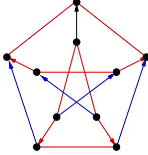
Figure 1: Any orientation of the Petersen graph has an NL-2-flow
